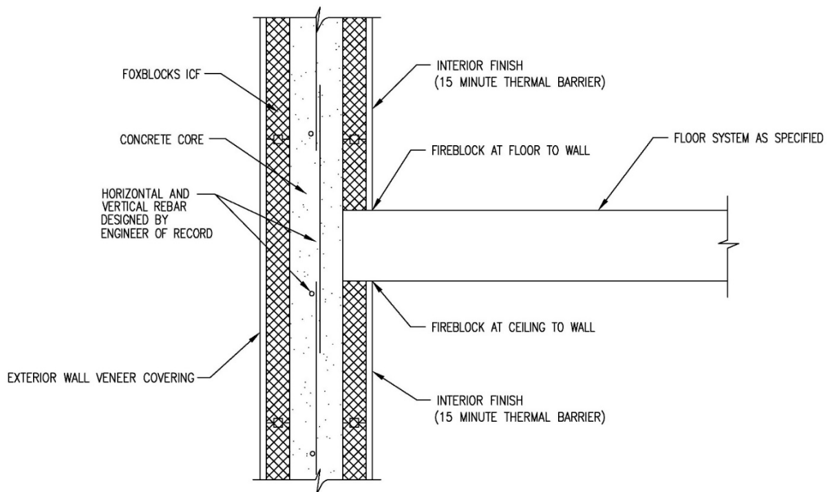
Figure 6 – TYPICAL WALL-TO-FLOOR INTERSECTION FOR TYPES I, II, III, AND IV CONSTRUCTION
