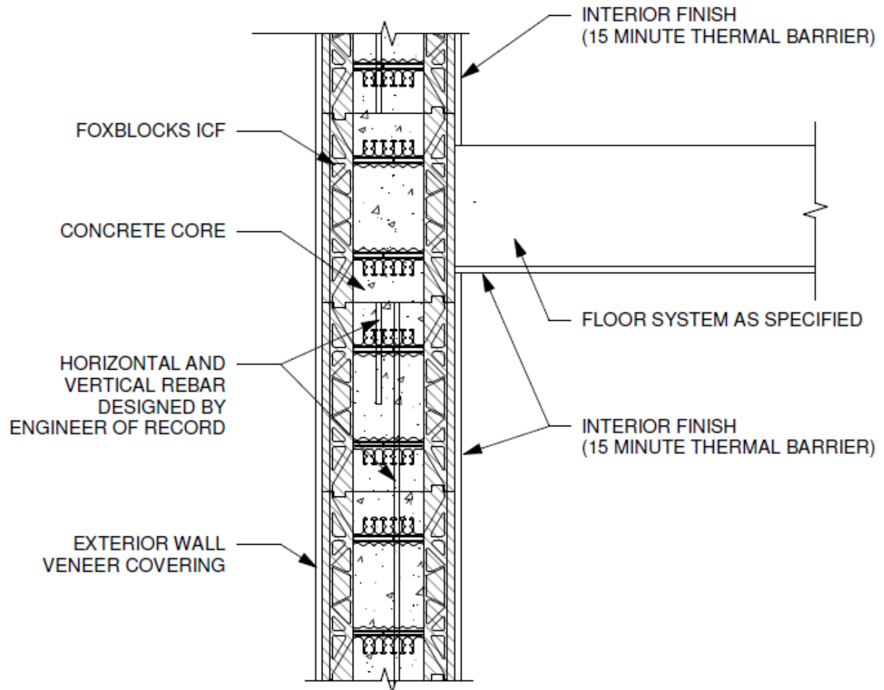
FIGURE 7 - TYPICAL WALL-TO-FLOOR INTERSECTION FOR TYPE V CONSTRUCTION
